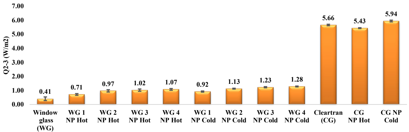
Fig. 6b: The comparison of the obtained heat flux for ZnS-SiO 2 NPs at 313 K
