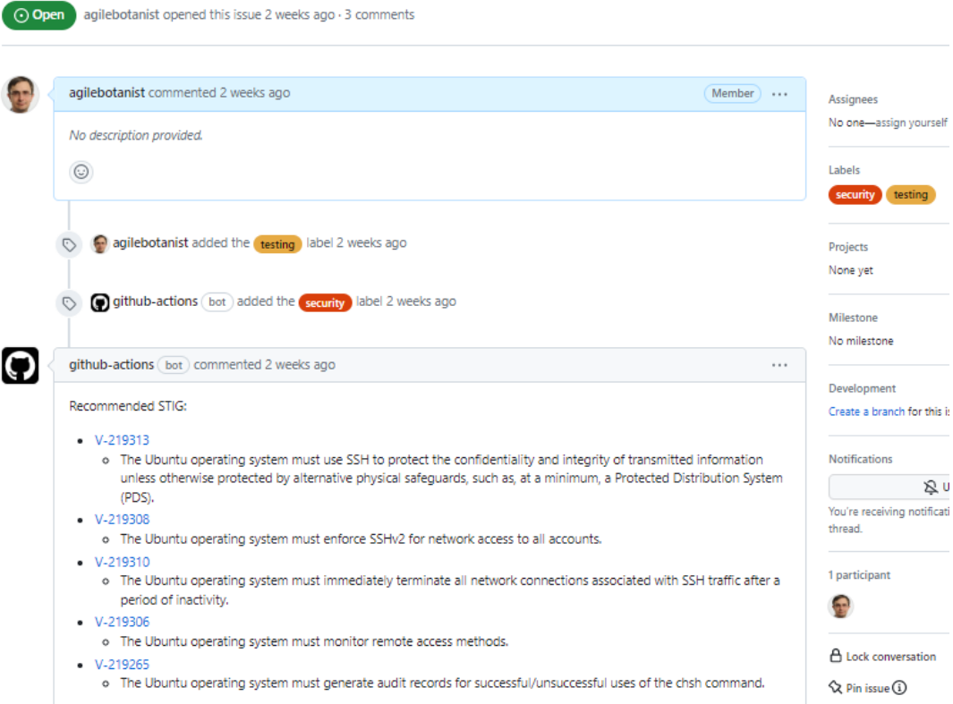
Figure 4: Automating Security Requirements Analysis with ARQAN
