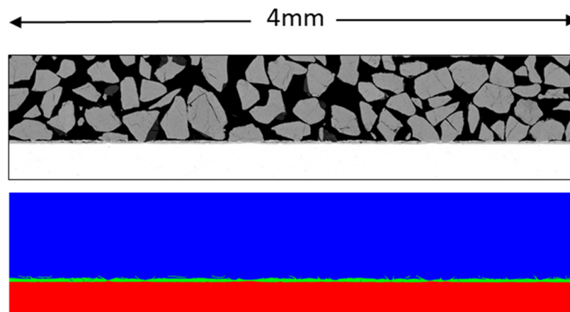
Figure 6. An example showing the back-scattered SEM image of 10CrMo9-10 cross-section (upper) and (lower) the colored cross-section of the same image showing the green-colored oxide layer between the metal (red) and deposit-epoxy mixture (blue).
