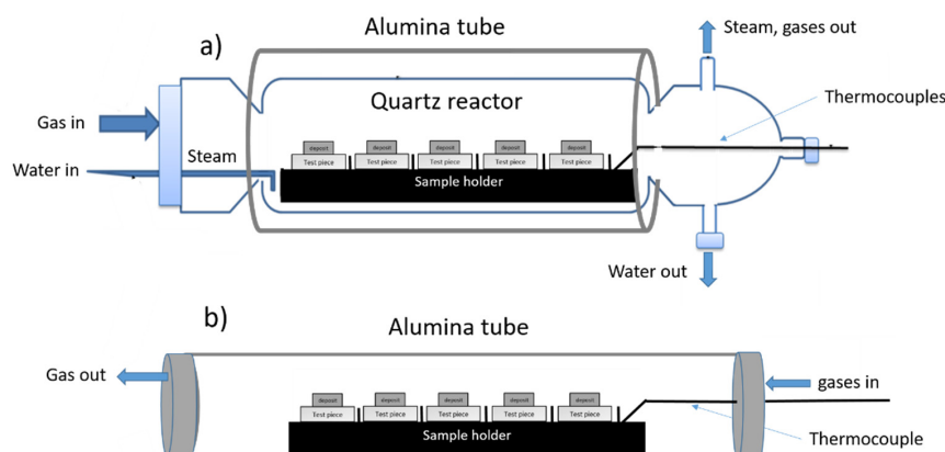
Figure 3. Quartz reactor and alumina tube used in experiments under (a) reducing and (b) oxidizing conditions.
