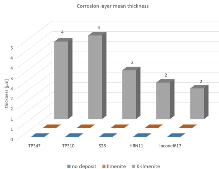
Figure 10. Mean thickness of oxide layer [µm] of samples exposed in dry air at 700 °C for 168 h.
