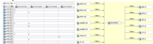
Figure 4: Example: Traceability links among the tool set, framework and case study requirements.
