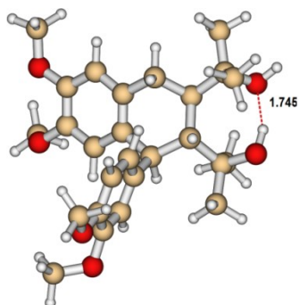
Figure 2. Energetically favored conformer of 9,9,9',9'-tetramethyl-dimethyl-cyclolariciresinol ( 4b ). The distance is given in Ångströms.
