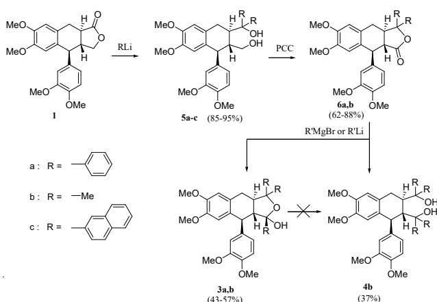
Scheme 2. Stepwise synthesis of the diols.
