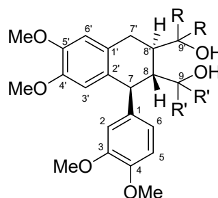
Figure 1. General structure and numbering of the sterically hindered 1,4-diol structures, represented by the substituted (R) aryltetralin 2'-7-cyclolignan dimethylcycloariciresinol.
