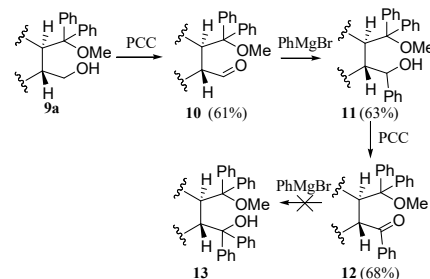
Scheme 4. Attempt to prepare a tetraphenyl substituted diol from the methyl protected compound 9a .
