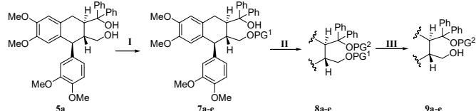
Scheme 3. Attempts to protect the more hindered OH group (O9'). Experimental conditions in Table 2 in Supporting Information.
