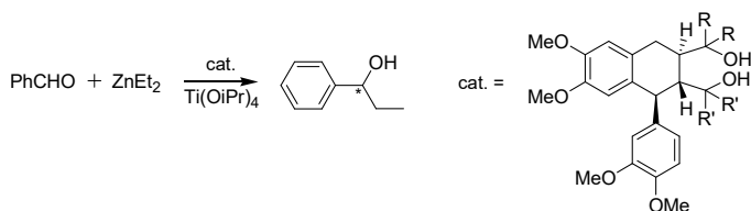
Scheme 5. Diethylzinc addition to benzaldehyde (test reaction).
