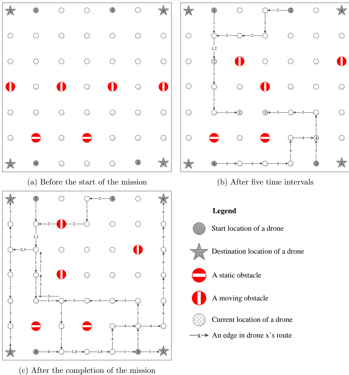
Figure 3: A simple illustrative example with four UAVs, two static obstacles, and four moving obstacles in a two-dimensional flying zone
