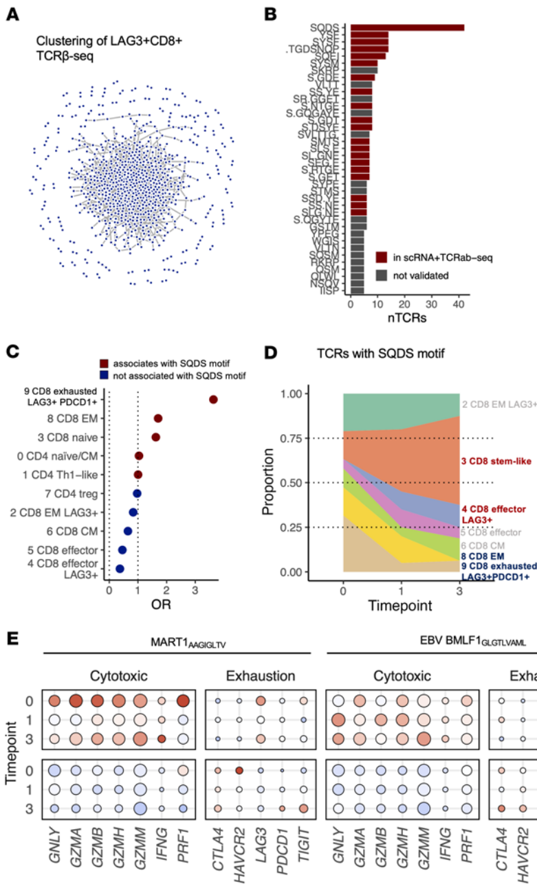
Figure 9. Anti-LAG-3+anti-PD-1 treatment invigorates LAG-3+CD8+ T cells targeting melanoma-associated antigens. (A) Network plot showing connections of similar TCRs in the LAG-3+CD8+-sorted TCRβ-Seq samples (n = 6), where a line between dots denotes amino acid-level similarities according to GLIPH2. (B) The number of clustered cells per TCR motif identified by GLIPH2 in the LAG-3+CD8+-sorted TCRβ-Seq samples, where the coloring indicates whether the motif was also identified in the analysis of TCRαβ-Seq data (n = 6, 18 samples). (C) ORs for TCRs with shared SQDS motifs showing a bias toward 9 CD8+ exhausted LAG3+PDCD1+ phenotypes. (D) A change in the phenotype of cells with the shared SQDS motif in their TCRs showed a decrease in the number of exhausted cells and an increase in cytotoxic cells in a responding patient. (E) Scaled average expression (avg.exp) and proportion of antigen-specific T cells (pct.exp) expressing canonical T cell markers in patients with CR/PR (n = 3) and PD (n = 3). Anti-MAA T cells were defined with TCRGP prediction against the MART1 AAGIGLTV target and against the antiviral EBV BMLF1 GLGTLVAML target.
