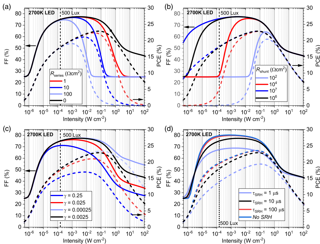
Figure 2. Fill factor (FF, solid curves, left axes) and power conversion efficiencies (PCEs, dashed curves, right axes) from drift–diffusion simulations based on a PM6:Y6 device with: a) Varying series resistance; b) varying shunt resistance; c) varying bimolecular recombination reduction factor; d) varying Shockley–Read–Hall (SRH) lifetime \tau_{SRH} .
