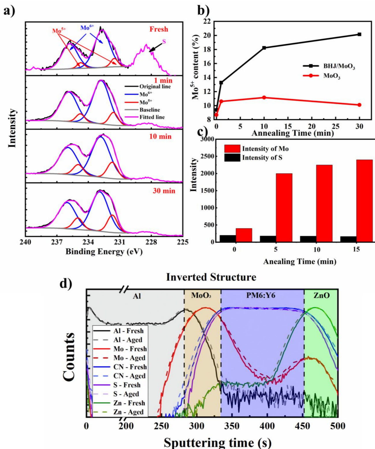
Figure 3. (a) XPS spectra of the Al/MoO 3 surface peeled from the cells after thermal annealed for different times; (b) change of Mo 5+ /(Mo 5+ + Mo 6+ ) of the Al/MoO 3 surface with different annealing times. The change of Mo 5+ content of the pure MoO 3 film upon thermal annealing was also included for comparison; (c) XPS signal intensity of Mo 3d and S 2s, which shows the almost identical S 2s intensity and increased Mo 3d intensity upon thermal annealing; (d) SIMS element distribution over the cell before and after thermal annealing for 30 min at 150 °C.
