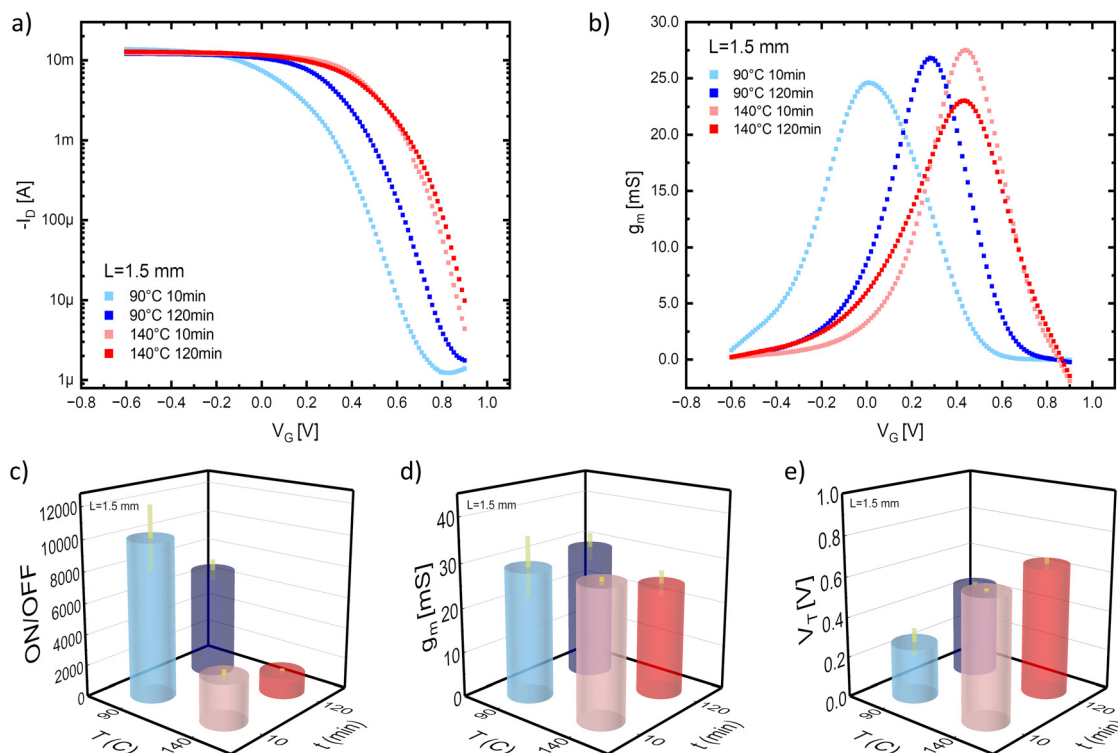
Fig. 2 Performance of OECTs with stencil size of L = 1.5 mm under varying annealing conditions. (A) Transfer curves of devices annealed at 90^\circ\text{C} (blue) and 140^\circ\text{C} (red) for 10 minutes (light) and 120 minutes (dark), V_D = -0.4 V. (b) Transconductance of devices, (c) on/off ratio with error bars (yellow lines), (d) Maximum transconductance, and (e) Threshold voltage, demonstrating the effect of temperature and time on the electrical properties of OECTs.
